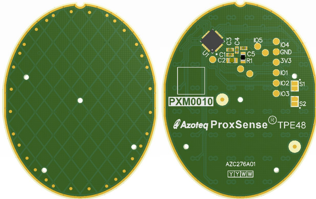
Figure 6.1 TPE48 – Module Representation.
