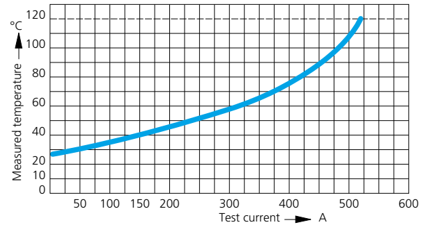
ODU Springtac® Socket Type 170-... Solid pin Type 180-... Contact Material Brass, silver-plated Contact-Ø 18 mm 240 mm² Cable Cross Section
