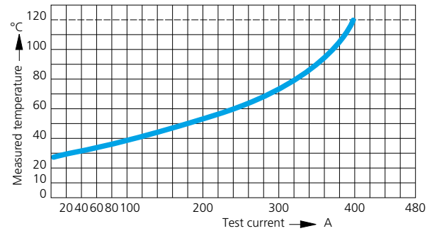
ODU Springtac® Socket Type 170-... Solid pin Type 180-... Contact Material Brass, silver-plated Contact-Ø 14 mm 150 mm² Cable Cross Section
