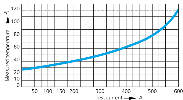
ODU Springtac® Socket Type 170-... Solid pin Type 180-... Contact Material Brass, silver-plated Contact-Ø 20 mm 300 mm² Cable Cross Section
