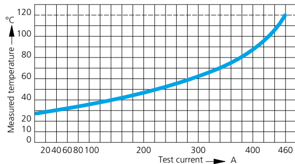
ODU Springtac® Socket Type 170-... Solid pin Type 180-... Contact Material Brass, silver-plated Contact-Ø 16 mm 185 mm² Cable Cross Section
