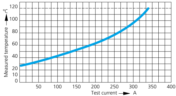
ODU Springtac® Socket Type 170-... Solid pin Type 180-... Contact Material Brass, silver-plated Contact-Ø 12 mm 95 mm² Cable Cross Section
