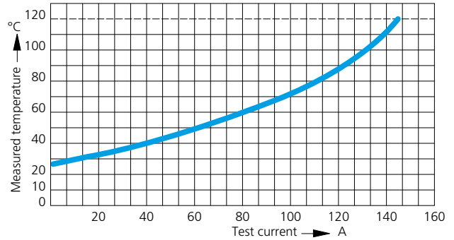
ODU Springtac® Socket Type 170-... Solid pin Type 180-... Contact Material Brass, silver-plated Contact-Ø 6 mm 25 mm² Cable Cross Section
