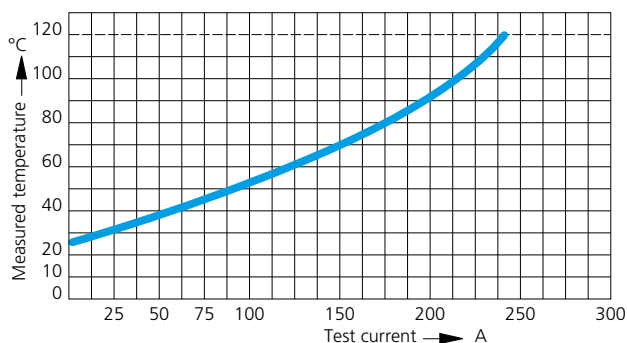
ODU Springtac® Socket Type 170-... Solid pin Type 180-... Contact Material Brass, silver-plated Contact-Ø 9 mm 50 mm² Cable Cross Section
