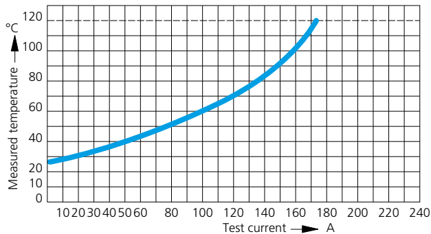
ODU Springtac® Socket Type 170-... Solid pin Type 180-... Contact Material Brass, silver-plated Contact-Ø 7 mm 35 mm² Cable Cross Section
