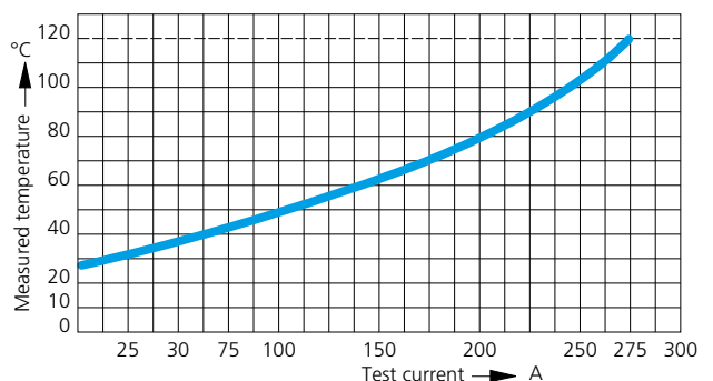
ODU Springtac® Socket Type 170-... Solid pin Type 180-... Contact Material Brass, silver-plated Contact-Ø 10 mm 70 mm² Cable Cross Section
