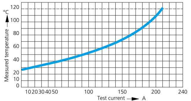
ODU Springtac® Socket Type 170-... Solid pin Type 180-... Contact Material Brass, silver-plated Contact-Ø 8 mm 50 mm² Cable Cross Section
