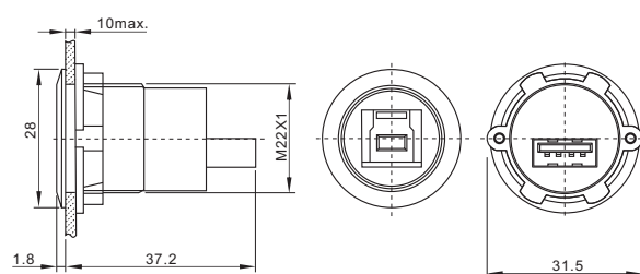
产品描述 : USB3.0 头部B型母/尾部A型母 Product Description: USB3.0 HEAD FEMALE B/BACK FEMALE A
