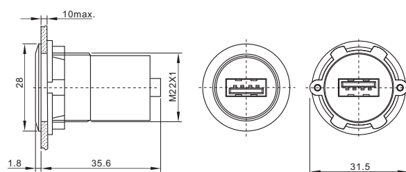
产品描述 : USB3.0 头部A型母/尾部A型母 Product Description: USB3.0 HEAD FEMALE A/BACK FEMALE A
