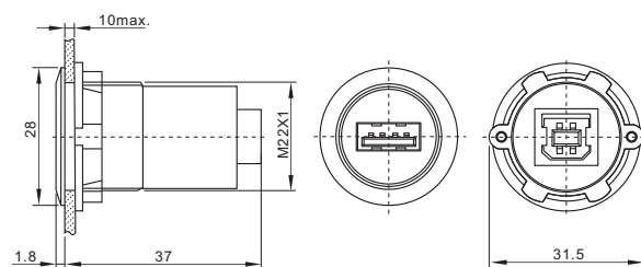
产品描述 : USB3.0 头部A型母/尾部B型母 Product Description: USB3.0 HEAD FEMALE A/BACK FEMALE B
