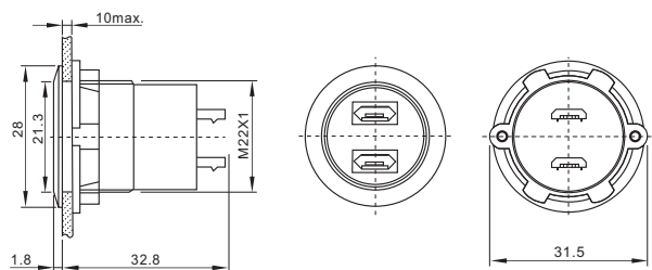
产品描述 : Micro USB2.0 头部2×B型母/尾部B型公 Product Description: Micro USB2.0 2×FEMALE B/ MALE B
